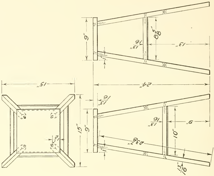
Kitchen Stool
